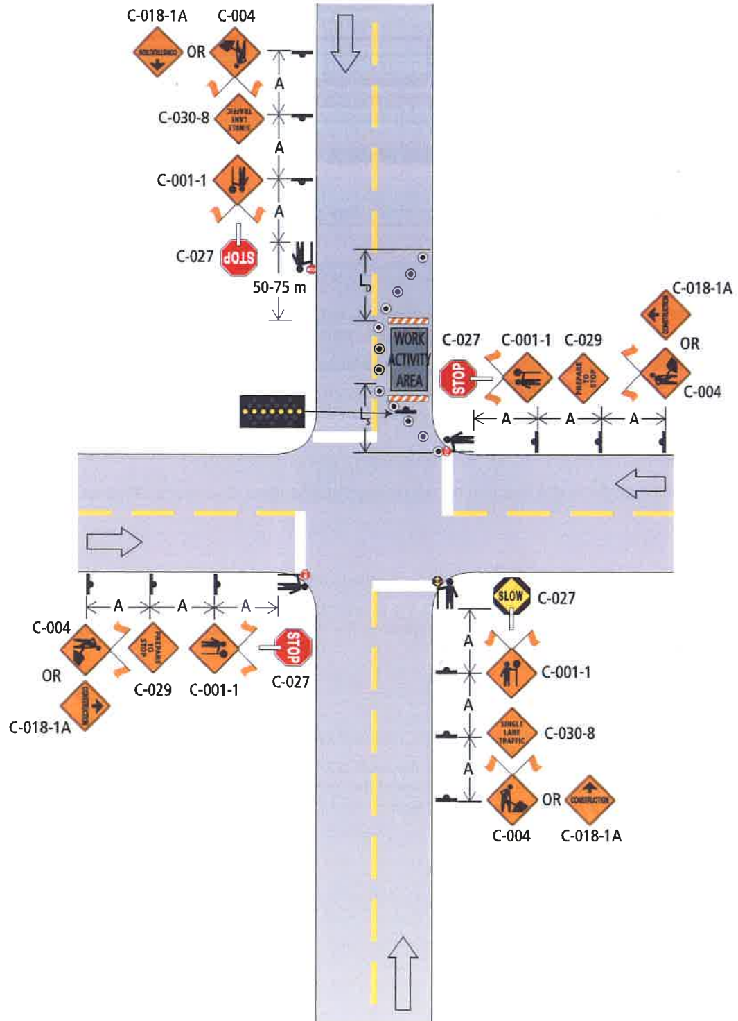
Figure 11.4: Intersection Lane Closure – Two-Lane, Two-Way Roadway with TCPs (Far Side) – Short and Long Duration
